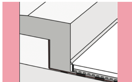
Installation on tiles
