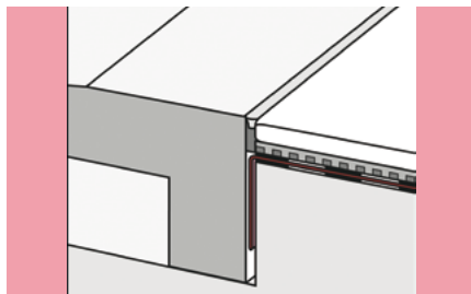
Installation floor-flush with tiles
