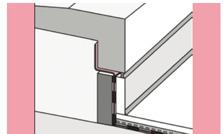
Installation on a base
